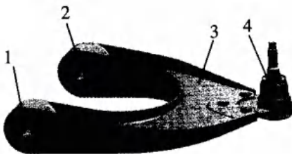
Fork arm 1 (1.2. Rubber bushing, 3. Arm body, 4. Ball joint assembly)
