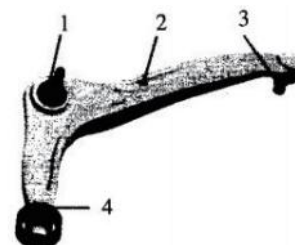
Single bushing, double ball hinge triangle arm. (1.3. Ball joint assembly, 2. Arm body, 4. Rubber bushing)
