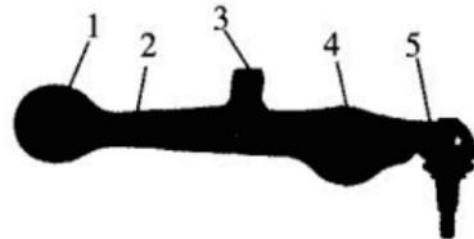
Support arm (1.4. Rubber bushing, 2. Control arm body, 3. Mounting hole, 5. Ball joint assembly)
