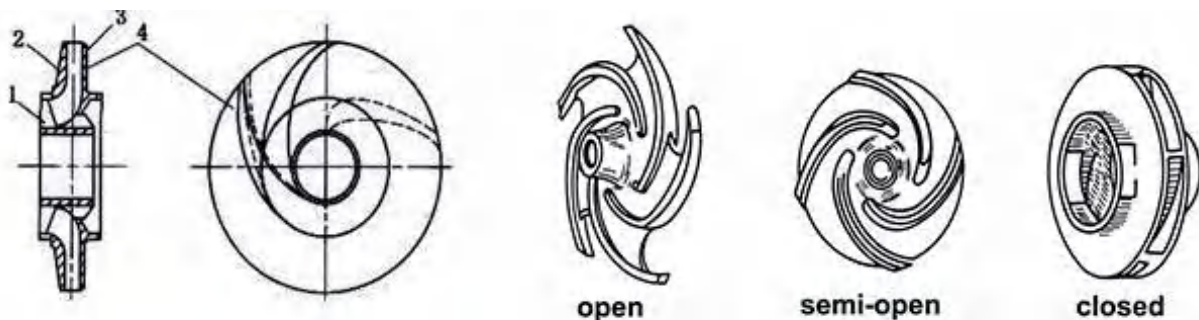
1-hub, 2-front cover, 3-rear cover, 4-blade
